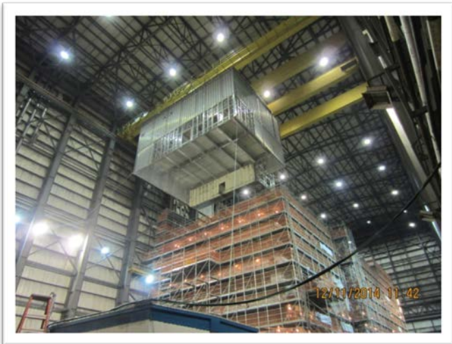
A fabricated block being lifted onto the living quarters.
